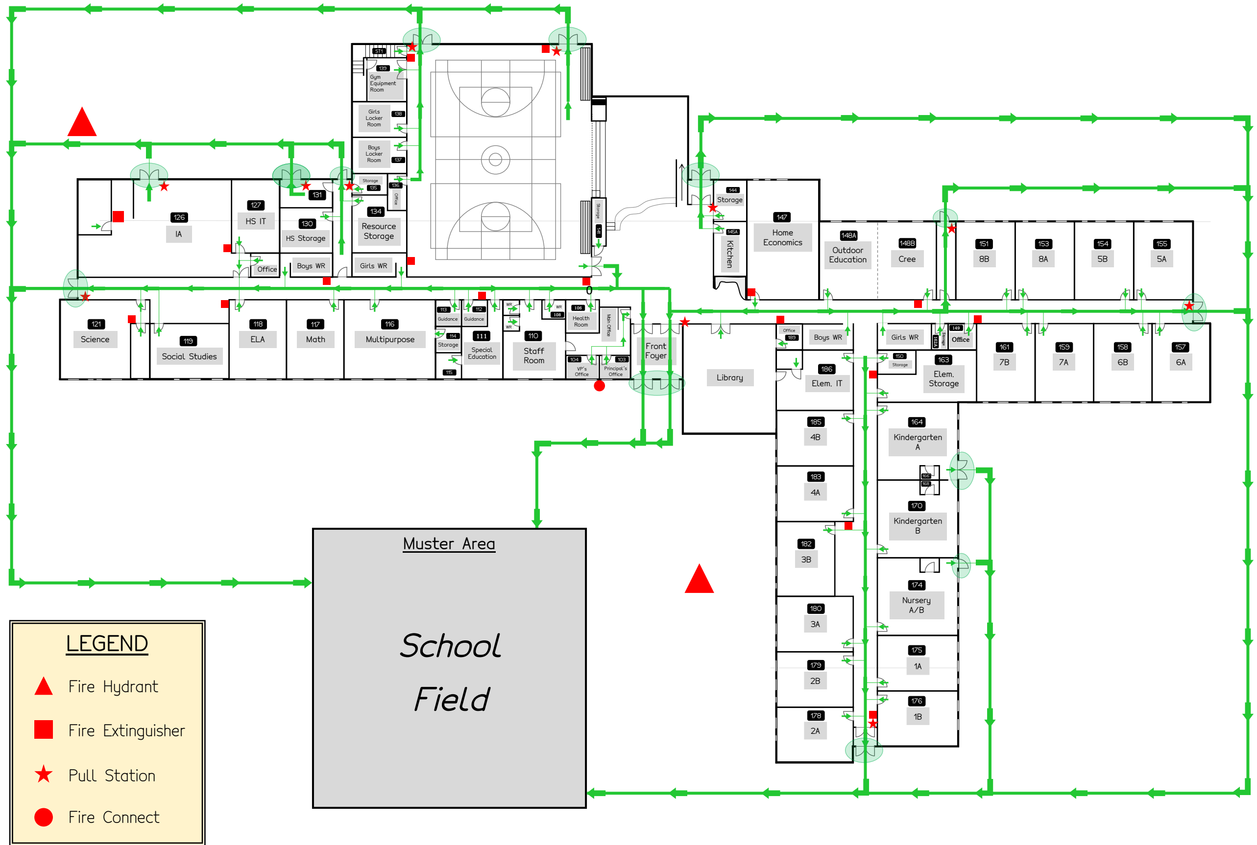
MSK Main Floor Plan
